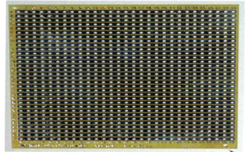
0.042" Dia. Holes on 0.100" Grid
